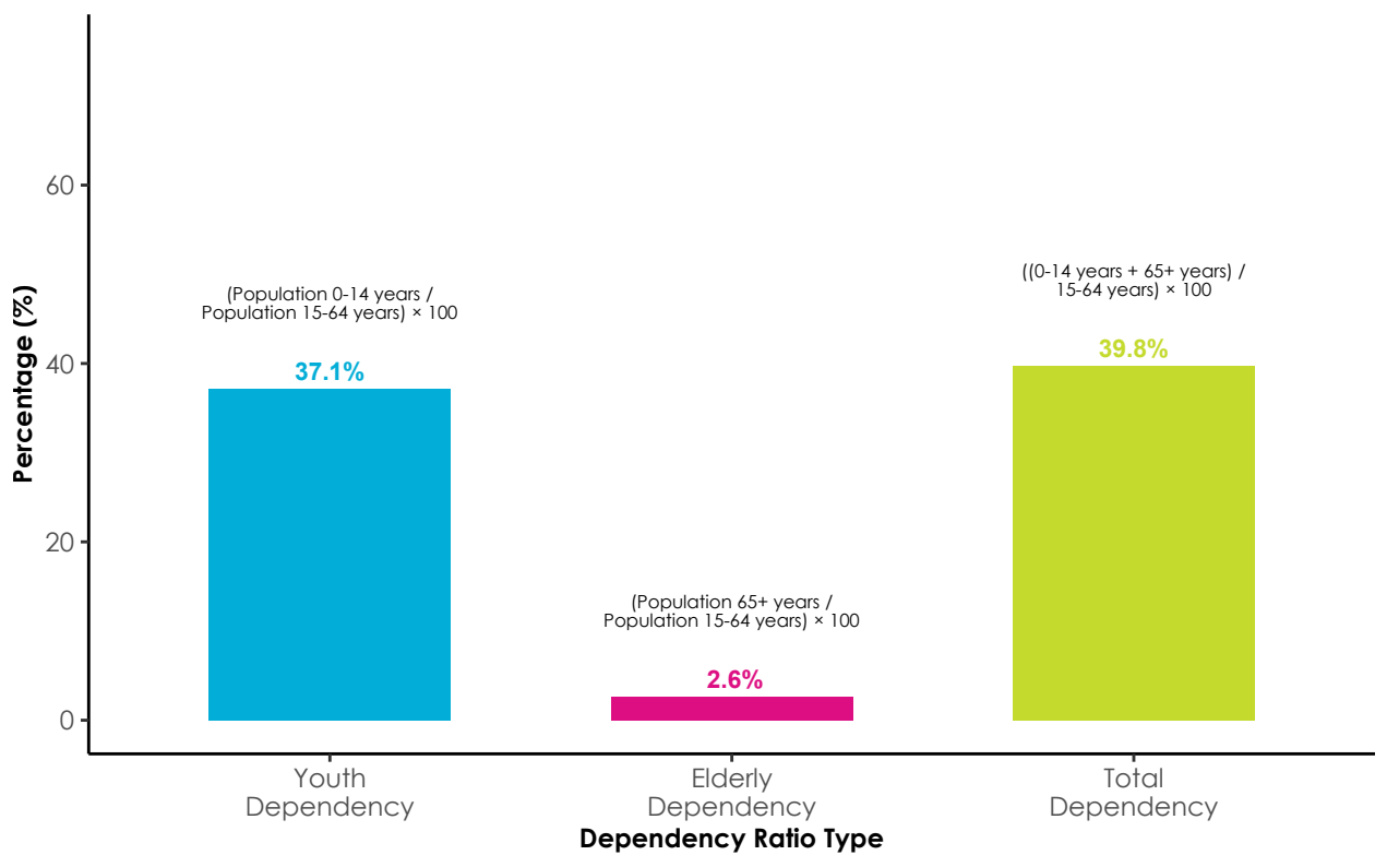
Figure 4: Dependency ratios (%)
