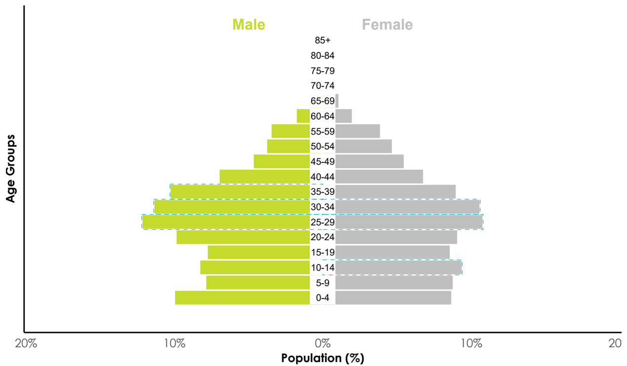
Figure 3: Population pyramid (%)
